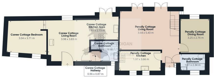
Floor 0 Building 1
